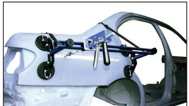
Wiggle Wire Dent Pulling
