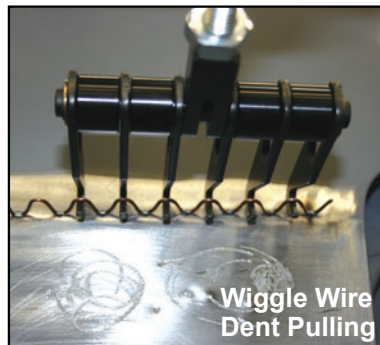
Pull Washer Dent Pulling
