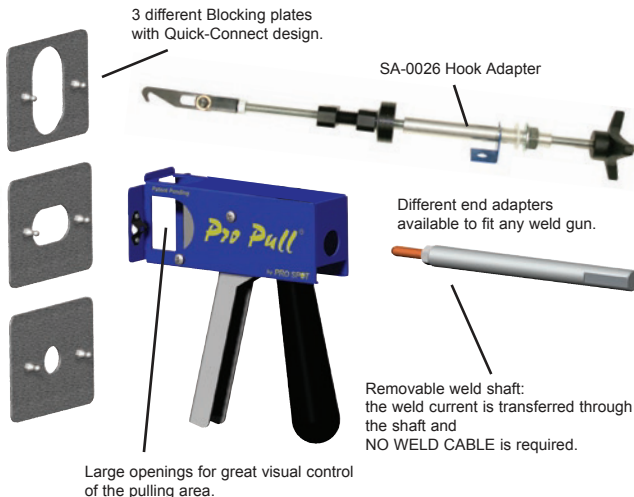
SA-0028 Single Pull System for Pro Pull
