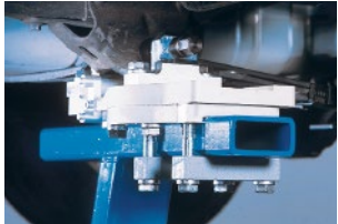
Truck clamping and holding is made easy with our B73 & B730 truck clamping kits
