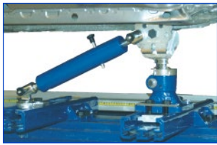
The EVO system locks parts in place when pulling, or holds them in place during welding operations
